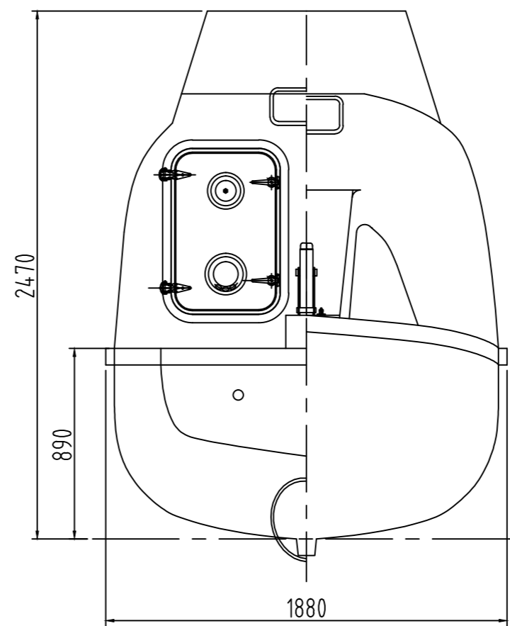
FRONT/AFT SECTION
